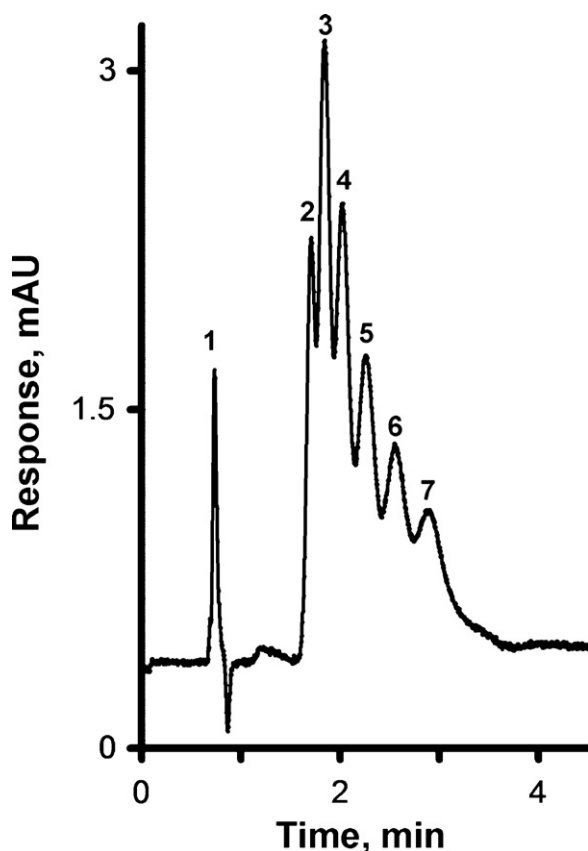
Fig. 3. Separation of uracil and alkylbenzenes using a monolithic poly(glycidyl methacrylate-co-ethylene dimethacrylate) capillary column with entrapped 0.25 wt% MWNT (with respect to the monomers) prepared at 55 °C. Conditions: column, 180 mm × 100 μm i.d., mobile phase 55% acetonitrile–5% THF–40% water, flow rate 1.00 μL/min, back pressure 17 MPa, UV detection at 254 nm; for peaks assignment see Fig. 2.
