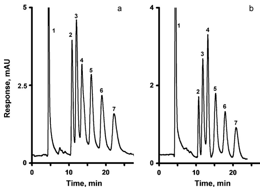
Fig. 9. Separation of uracil and alkylbenzenes using a monolithic poly(glycidyl methacrylate- co -ethylene dimethacrylate) capillary column prepared at 70 °C and modified with ammonia followed by attachment of oxidized MWNT. Conditions: column, 170 mm × 100 μm i.d., mobile phase 50% acetonitrile–50% water (a) and a 47.5% acetonitrile–2.5% THF–50% water–mixture (b); flow rate 0.25 μL/min, back pressure 30 MPa; UV detection at 254 nm; for peaks assignment see Fig. 2.
