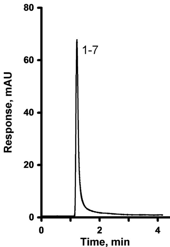
Fig. 7. Separation of uracil and alkylbenzenes using a monolithic poly(glycidyl methacrylate-co-ethylene dimethacrylate) capillary column prepared at 55 °C and modified with ammonia. Conditions: column, 200 mm × 100 μm i.d., mobile phase 50% acetonitrile–50% water, flow rate 1.00 μL/min, back pressure 17 MPa, UV detection at 254 nm; for peaks assignment see Fig. 2.
