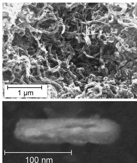
Fig. 4. SEM image of pristine 1–2 μm long MWNT aggregated after exposure to water (top) and SEM micrograph of oxidatively cut MWNT.
